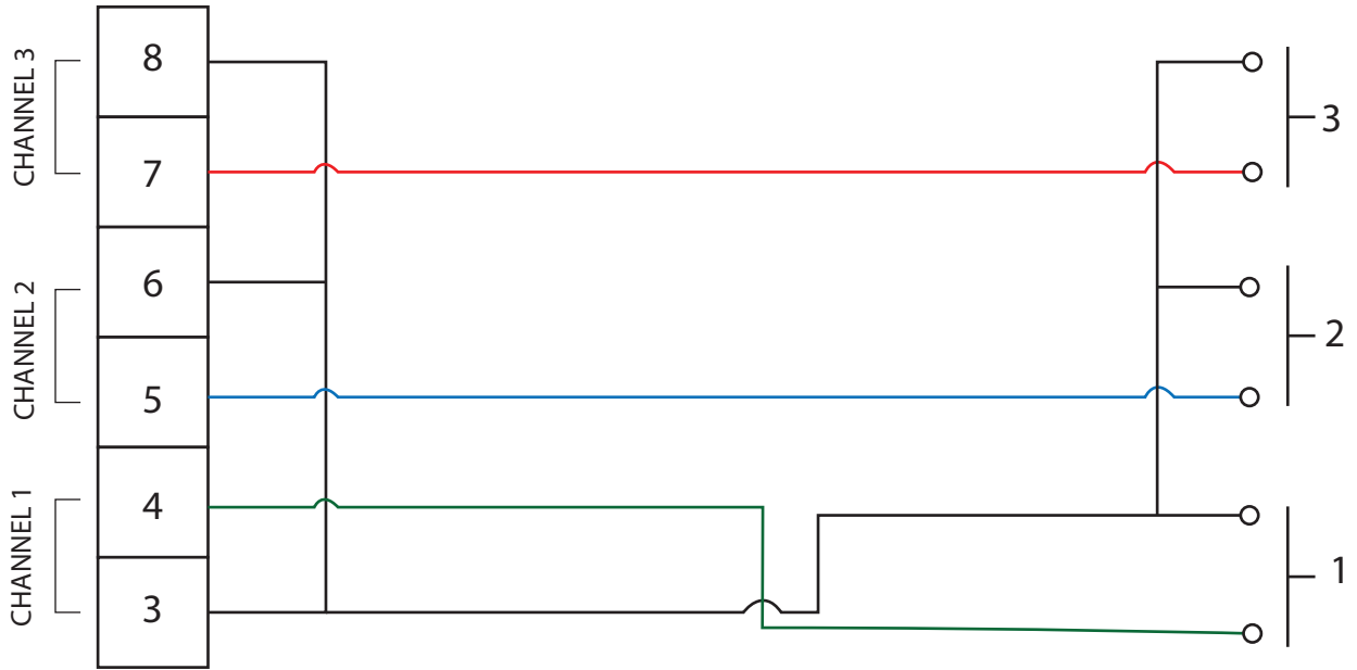
DIAGRAM FOR 4 WIRES
